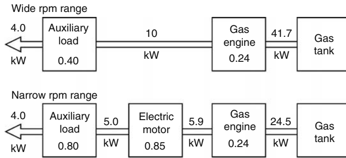
FIGURE 5.3 Shifting the auxiliary load from the engine to an electrical motor.
