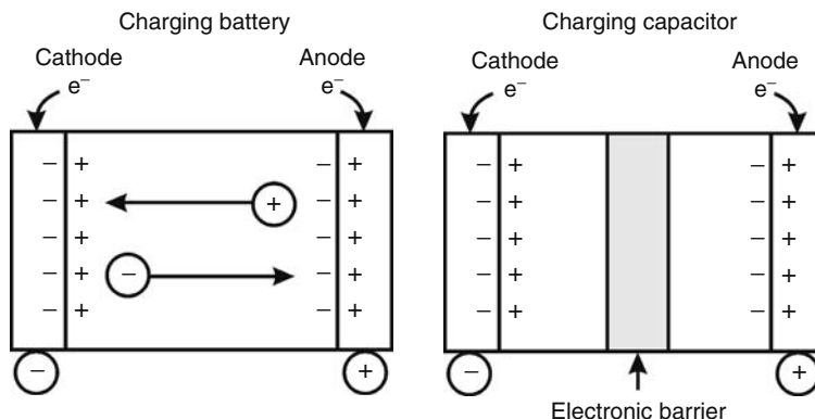
FIGURE 6.20 Comparison of battery and SC.
