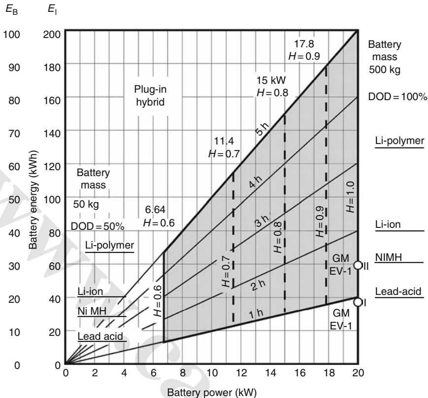
FIGURE 6.15 Box for adequate power but large energy; the expanded box for the PHEV of Figure 6.14.
