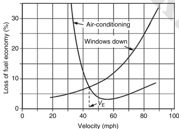
FIGURE 12.19 Percent fuel economy loss as a function of vehicle velocity for A/C and added aerodynamic drag due to windows down for ventilation. Also, illustration of the equal velocity, V_E .
