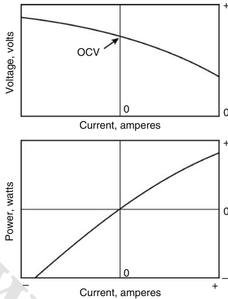
FIGURE A.6.8 Voltage and power during the discharging and the charging of a cell.
