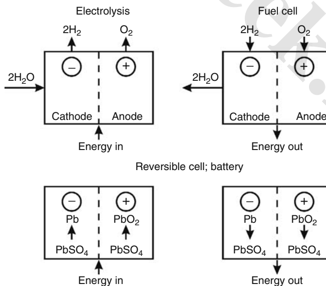
FIGURE 6.17 Differences between reversible cells and FCs.
