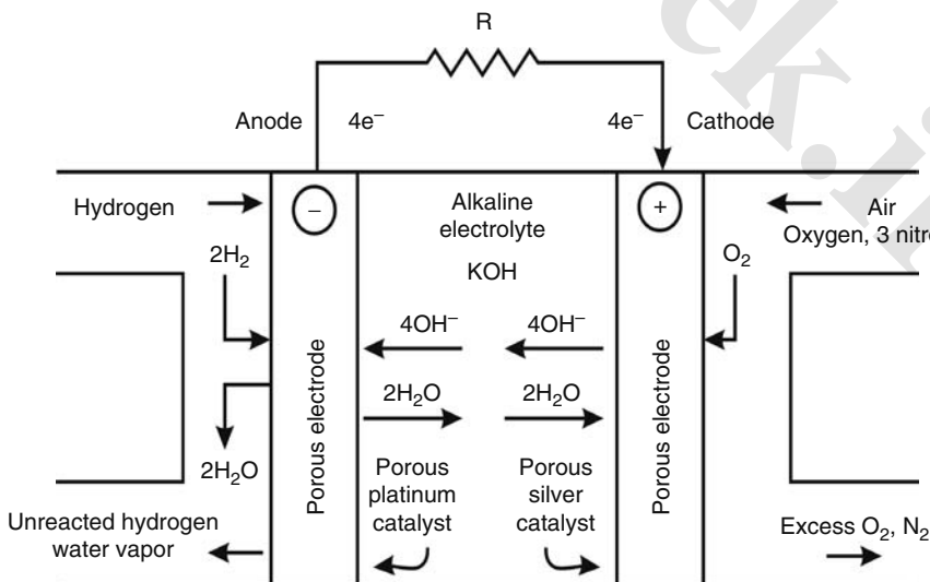
FIGURE A.6.9 Hydrogen/oxygen FC with an alkaline electrolyte, KOH.
