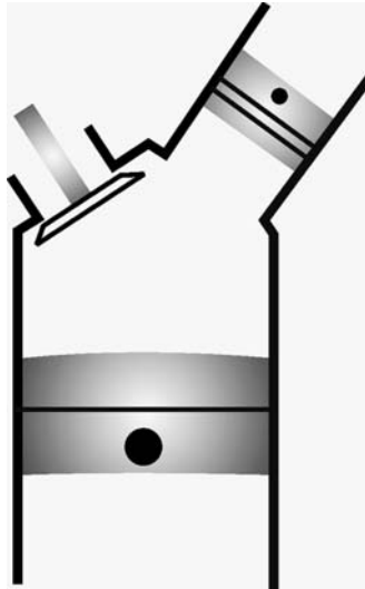
FIGURE 17.8 Combustion chamber of an Alvar engine. The small piston has a crankshaft separate from the crankshaft of main piston. An electrical motor drives the crankshaft for the small piston. (Reprinted with permission from SAE Paper Advanced Vehicle Powertrains 2005 , SP-1973, © 2005 SAE International.)
