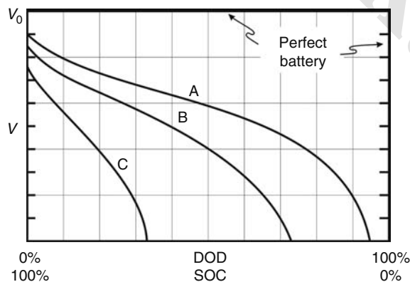
FIGURE 6.2 Voltage at the battery terminals depending on the SOC. Curves A, B, and C are for different discharge electrical currents.
