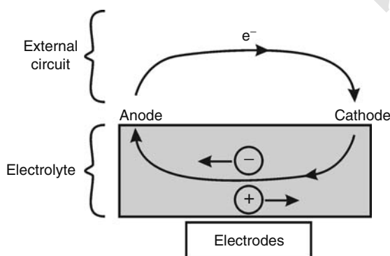
FIGURE A.6.1 Nomenclature for the electrodes. This is a circuit for a cell which is converting chemical energy to electrical energy. The motion of negative charges is clockwise and forms a closed loop through external wires and load and the electrolyte in the cell.
