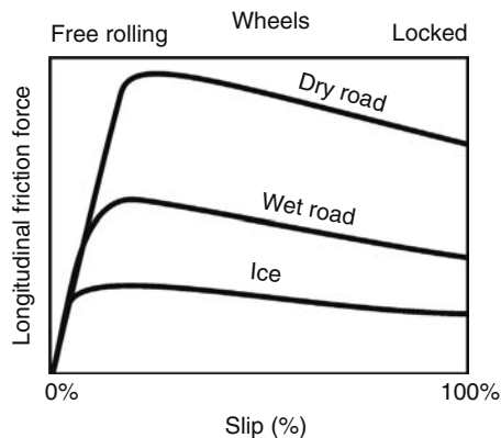
FIGURE 9.6 Friction force because of braking as a function of longitudinal slip for three different road surfaces: dry road, wet road, and ice.
