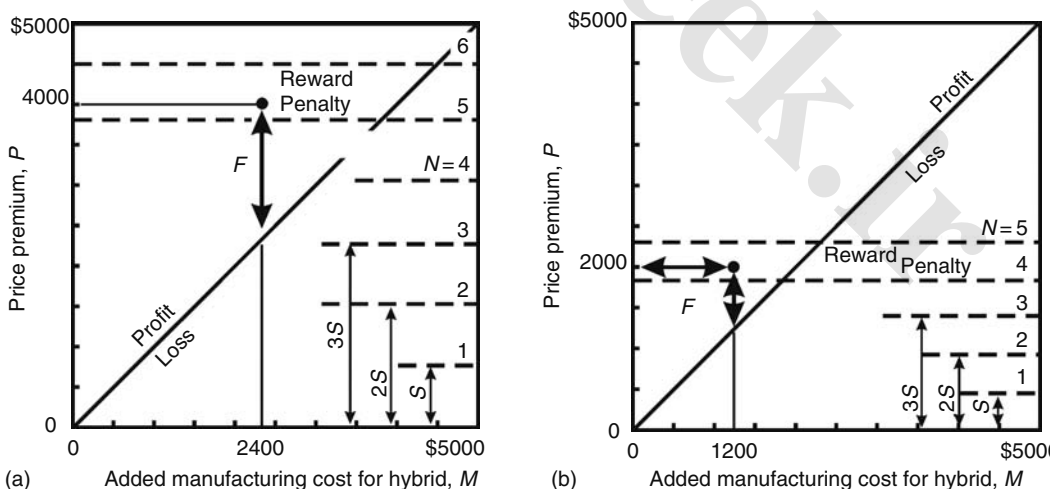
FIGURE 15.4 Effect of mild and full hybrid designs on profit/loss for the manufacturer and reward/penalty for the customer. (a) Point for a full hybrid in the P, M coordinates. Numerical values for the graph are S = \$750/\text{year} , P = \$4000 , and M = 0.6 , P = \$2400 . Profit, F , is $1600. (b) Point for a mild hybrid in the P, M coordinates. Numerical values for the graph are S = \$450/\text{year} , P = \$2000 , and M = 0.6 , P = \$1200 . Profit, F , is $800.
