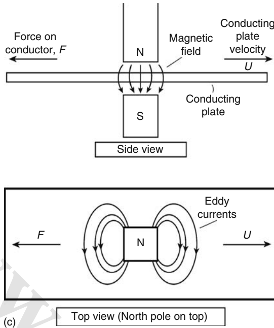
FIGURE 14.2 (continued) (c) Eddy currents are created (induced) by motion of the conducting plate through the magnetic field. The eddy currents interact with the magnetic field and cause a force in a direction opposing conductor motion. An example using this force is an inductance motor.
