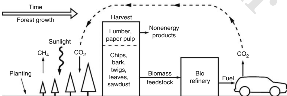
FIGURE 22.6 \text{CO}_2 cycle; fuel from biomass.
