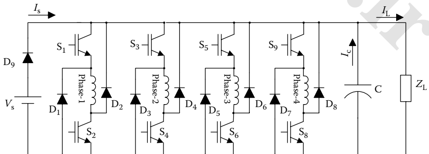
FIGURE 6.68 A driving circuit example for the SRG.
