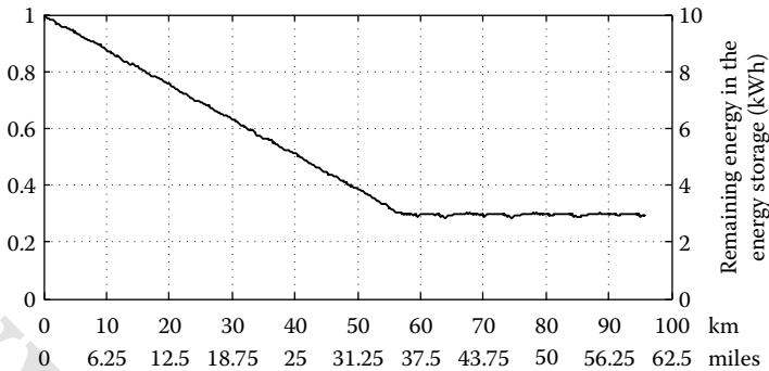
FIGURE 10.19 SOC and the remaining energy in the energy storage versus traveling distance in FTP75 urban driving cycle with CD mode.
