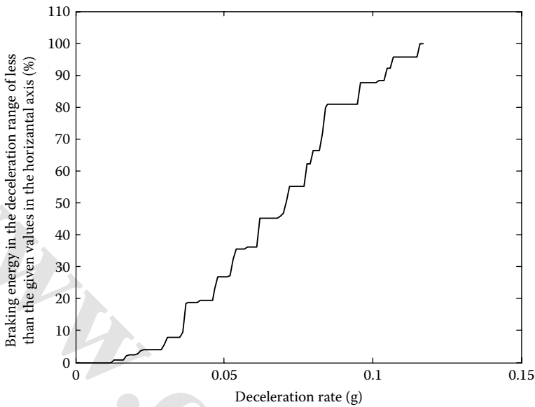
FIGURE 13.8 Braking energy dissipated in various vehicle deceleration rates.
