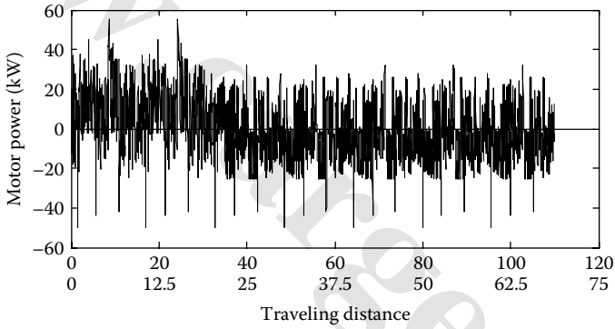
FIGURE 10.11 Motor power versus traveling distance in LA92 driving cycle with AER mode.
