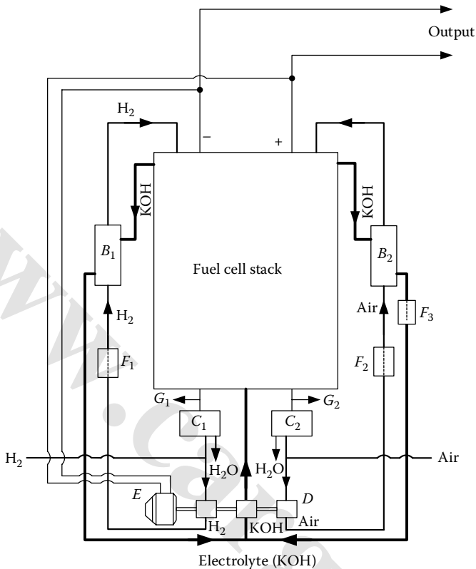
FIGURE 14.7 Circulating electrolyte and supplies of hydrogen and air in an AFC; B_1 , B_2 , heater exchangers; C_1 , C_2 , condensers; D , pumpers; E , motor; F_1 , F_2 , F_3 , controls; and G_1 , G_2 , outlets. 8
