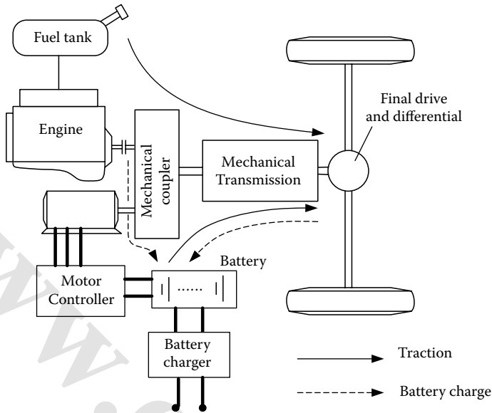
FIGURE 5.5 Configuration of a parallel hybrid electric drive train.
