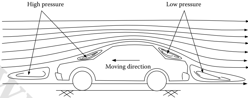
FIGURE 2.5 Shape drag.
