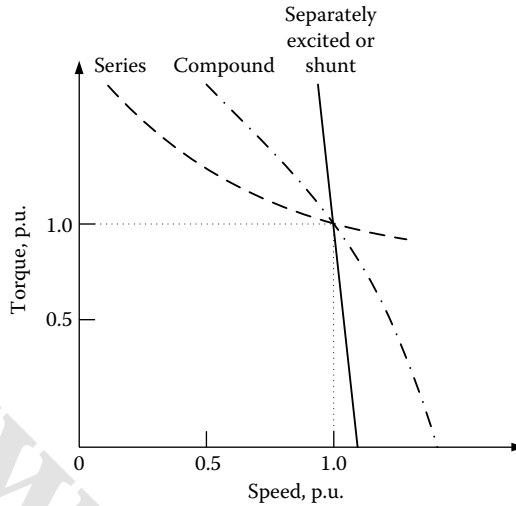
FIGURE 6.6 Speed characteristics of DC motors.
