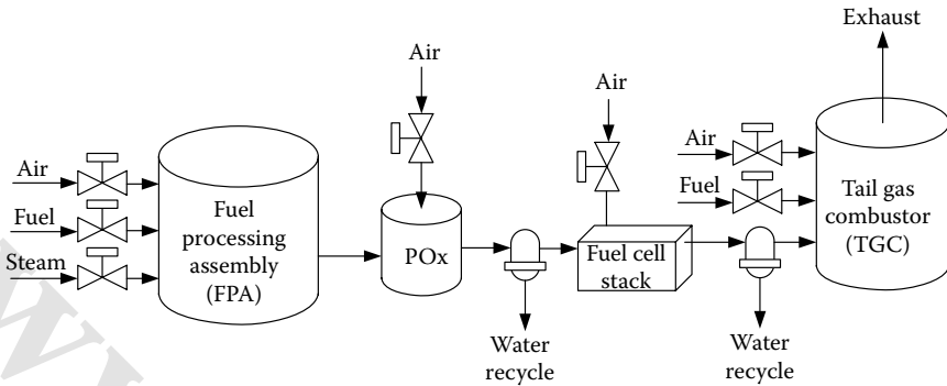
FIGURE 14.11 Fuel processing diagram. 13
