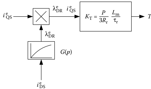
FIGURE 6.26 Block diagram of a field-orientated induction motor.
