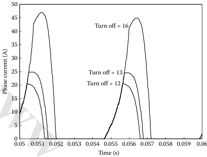
FIGURE 6.69 Effect of the turn-off angle in maximum current level in generating mode in an 8/6 switched reluctance machine.
