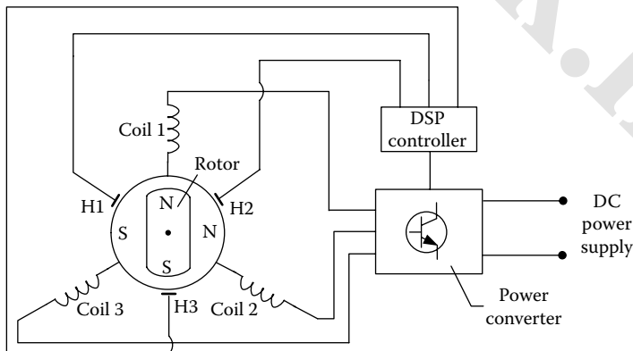
FIGURE 6.42 BLDC motor.
