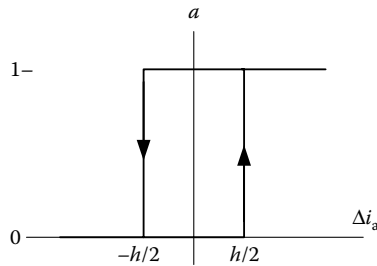
FIGURE 6.39 Input–output characteristics of a hysteresis current controller.
