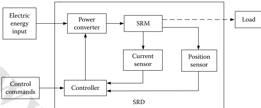
FIGURE 6.54 SRM drive system.
