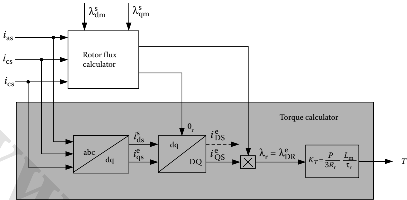
FIGURE 6.31 Torque calculator.
