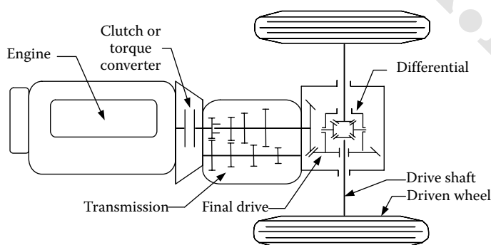
FIGURE 2.10 Conceptual illustration of an automobile power train.
