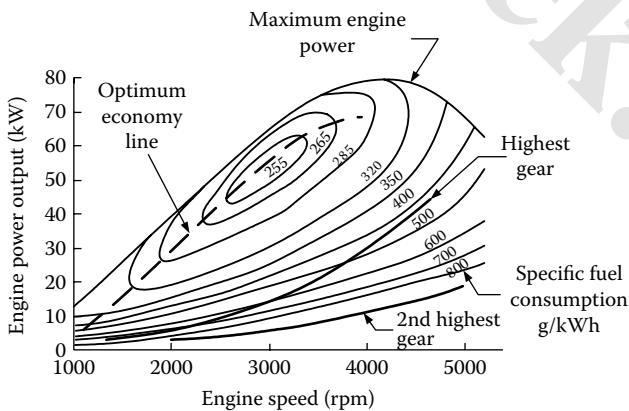
FIGURE 2.32 Operating point of the engine at a constant speed with highest gear and second highest gear.
