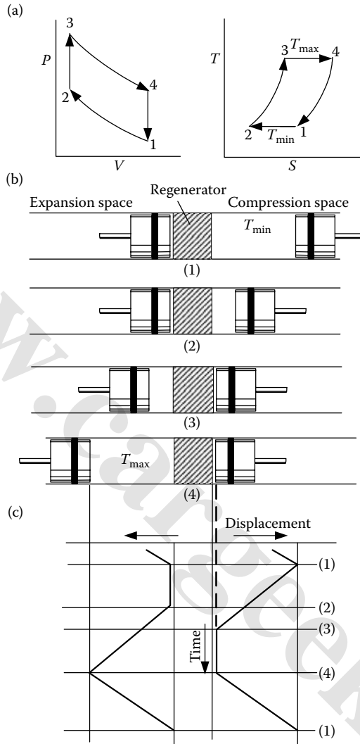
FIGURE 3.17 Ideal Stirling cycle: (a) P - V and T - S diagram, (b) piston arrangement at the terminal points of the cycle, and (c) time-displacement diagram.
