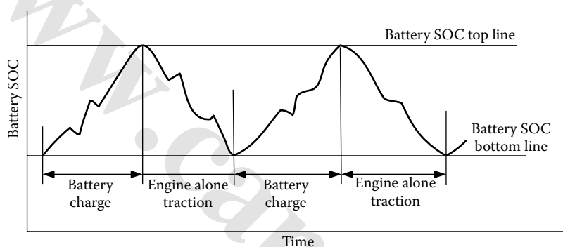
FIGURE 11.4 Battery charge and engine-alone traction, depending on the battery SOC.
