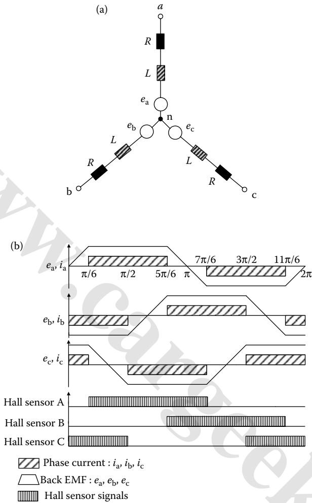
FIGURE 6.45 (a) Three-phase equivalent circuit and (b) back EMFs, currents, and Hall sensor signals of a BLDC motor.
