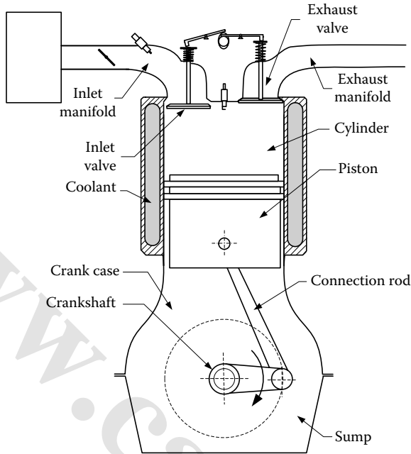
FIGURE 3.1 4S, SI gasoline engine.
