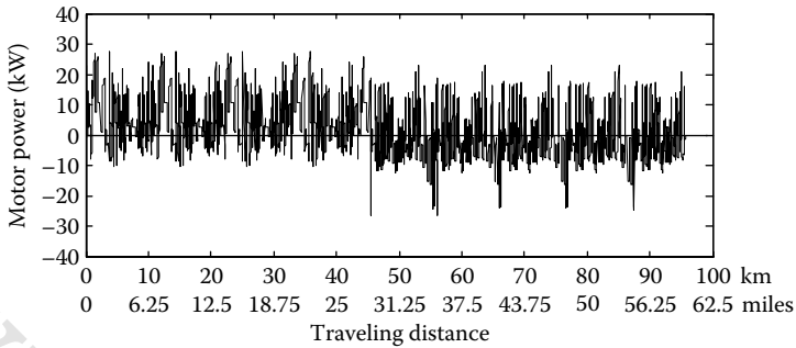
FIGURE 10.5 Motor power versus traveling distance in FTP75 urban driving cycle with AER mode.
