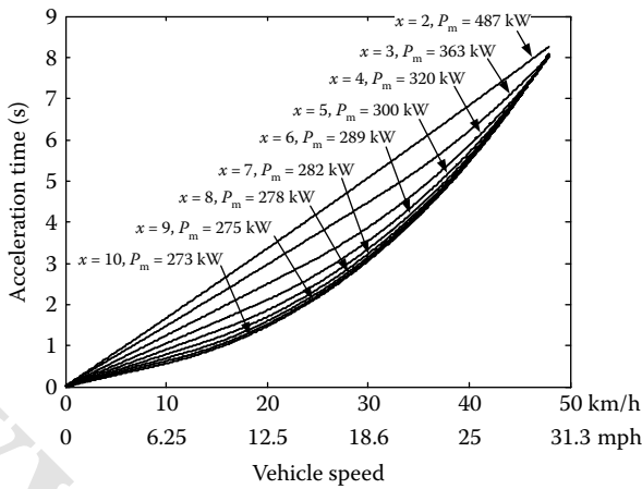
FIGURE 16.7 Motor power required by acceleration performance with different extended speed ratios, x .
