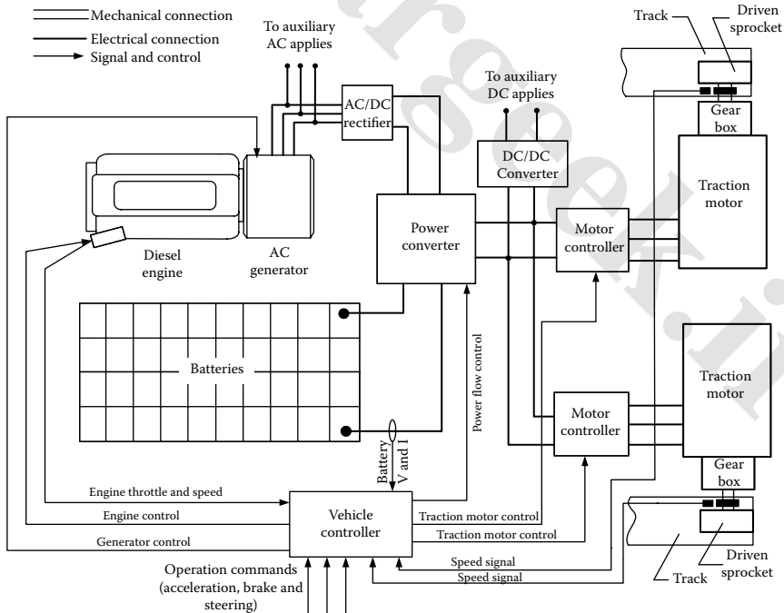
FIGURE 16.4 Tracked series hybrid off-road vehicle architecture.
