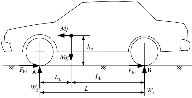
FIGURE 2.38 Force acting on a vehicle during braking on a flat road.
