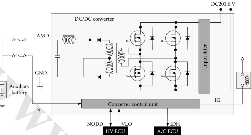
FIGURE A.6 DC-DC converter.
