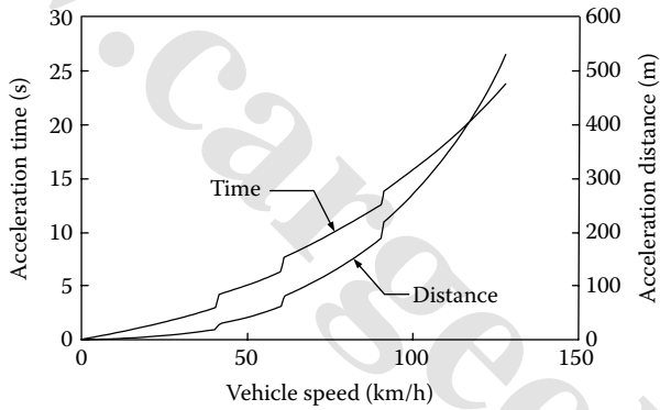
FIGURE 2.28 Acceleration time and distance along with vehicle speed for a gasoline-engine-powered passenger car with four-gear transmission.
