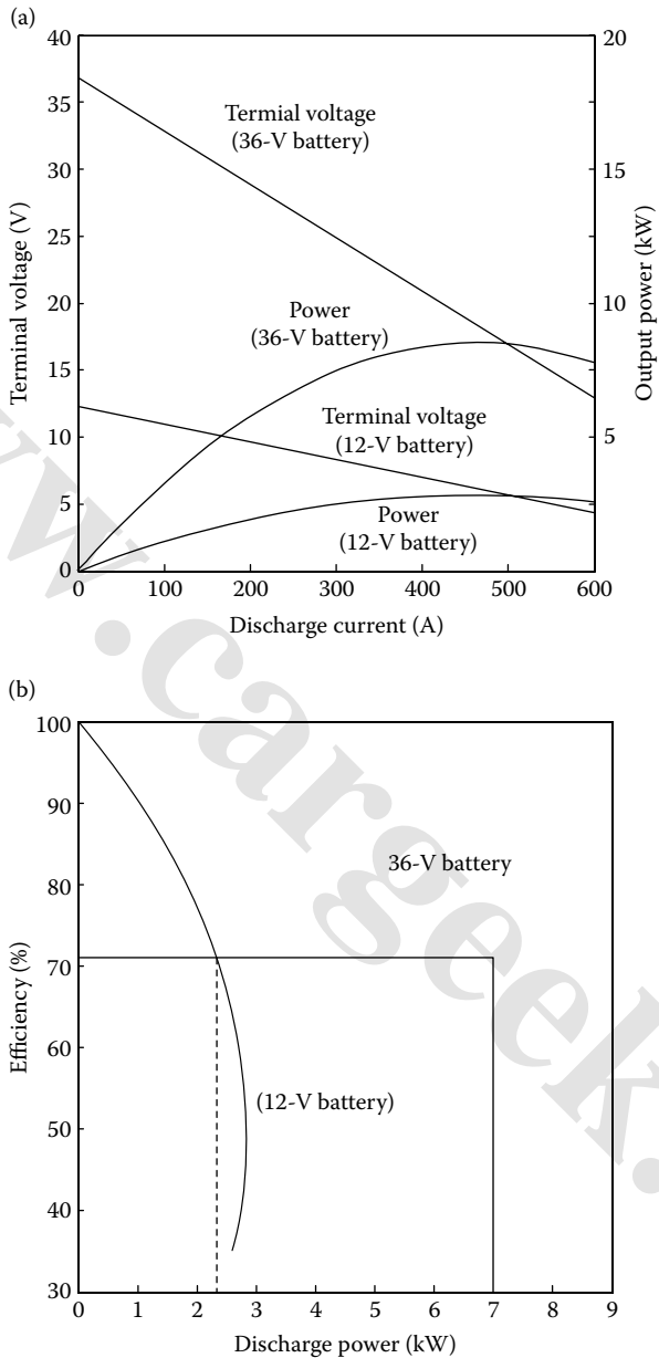
FIGURE 11.9 Battery performance with 36 and 12 V rated voltages: (a) battery power and terminal voltage versus discharge current and (b) battery discharge efficiency.
