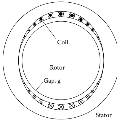
FIGURE 6.46 Winding configuration of sinusoidal-shaped back EMF BLDC.
