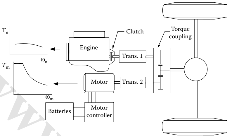
FIGURE 5.8 Two-shaft configuration.
