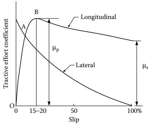
FIGURE 2.8 Variation of tractive effort coefficient with longitudinal slip of a tire.
