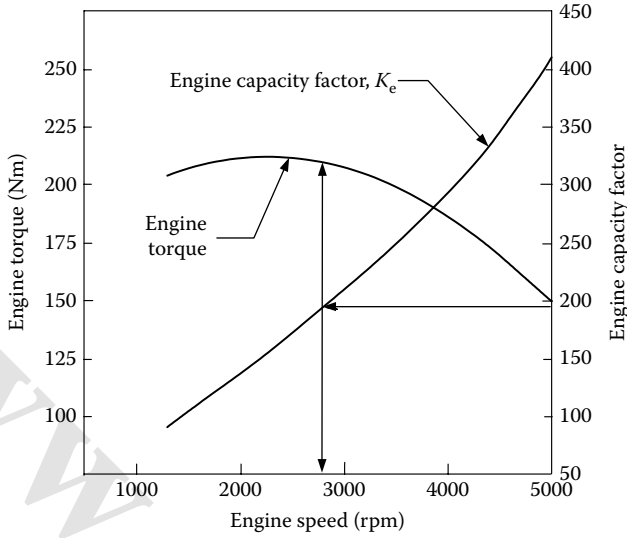
FIGURE 2.22 Capacity factor of a typical engine.
